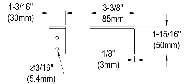
Bracket (2 pcs) Scale 2:1
